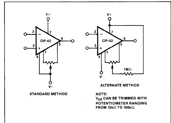
FIGURE 3: Input Offset Voltage Nulling
