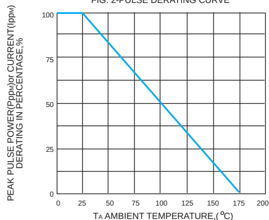
FIG. 2-PULSE DERATING CURVE
