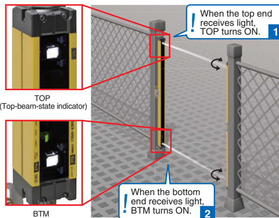
BTM (Bottom-beam-state indicator)
