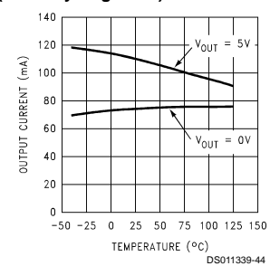
Current Limit vs Temperature (Auxiliary Regulator)
