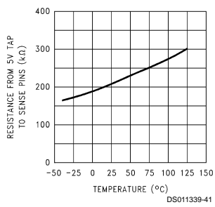
Divider Resistance
