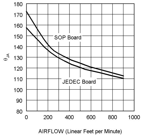
FIGURE 3. \theta_{JA} vs Airflow
