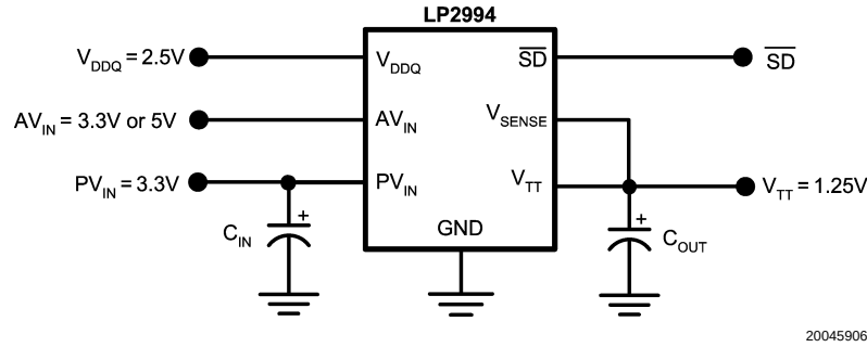
FIGURE 6. SSTL-2 Implementation with higher voltage rails
