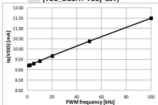
Figure 21. Quiescent current I q (VDD) (T=25°C; no fault; [VDD-VSS]=25V)
