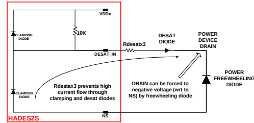
Figure 24: DESAT clamping circuit
