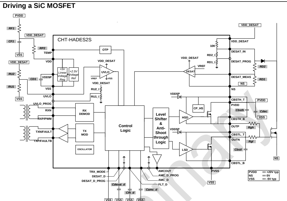
Figure 32: Typical application schematic (SiC MOSFET power device)
