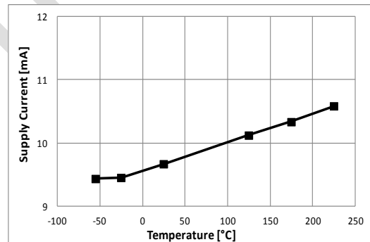
Figure 20. Quiescent current I q (VDD) (20 kHz; no fault; [VDD-VSS]=25V)
