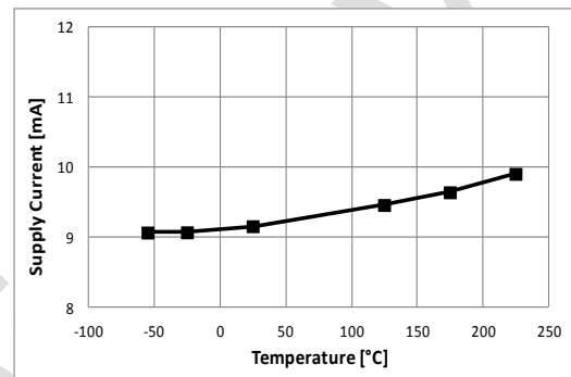
Figure 18. Quiescent current I q (VDD) (0 Hz; no fault; [VDD-VSS]=25V)
