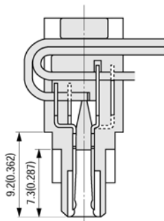
X-X' Cross Section
