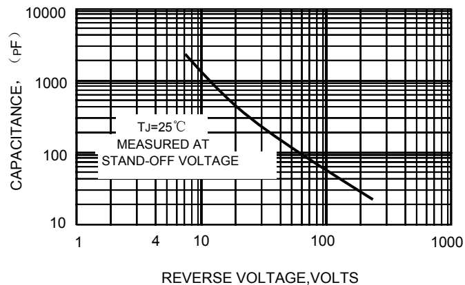
FIG.2-TYPICAL JUNCTION CAPACITANCE
