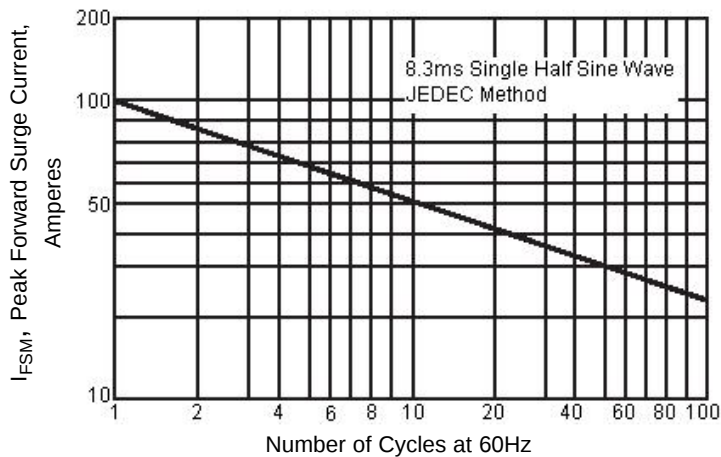
Maximum Non-Repetitive Forward Surge Current Unidirectional Only
