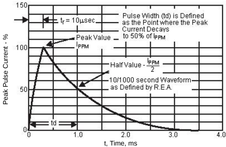
Clamping Power Pulse Waveform
