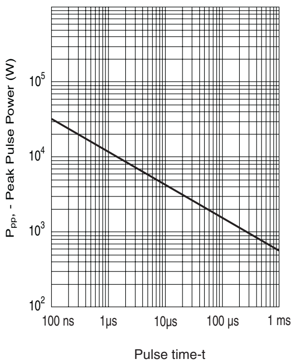
PEAK PULSE POWER RATING CURVE
