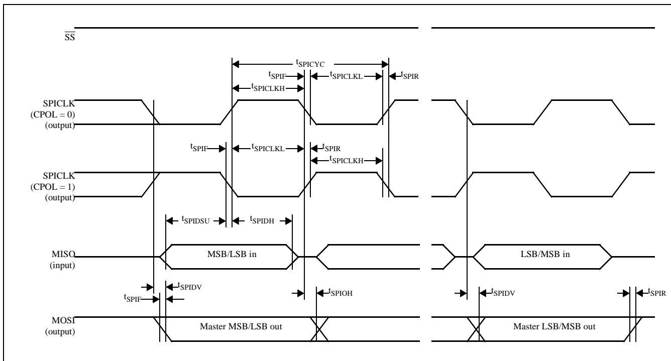
Figure 8: SPI Master Timing (CPHA = 0)
