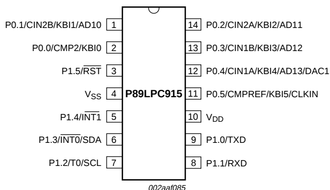
Fig 8. P89LPC915 DIP14 pin configuration
