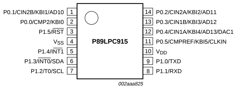
Fig 7. P89LPC915 TSSOP14 pin configuration
