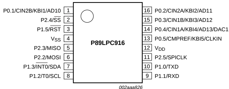
Fig 9. P89LPC916 TSSOP16 pin configuration
