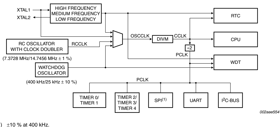
Fig 5. Block diagram of oscillator control
