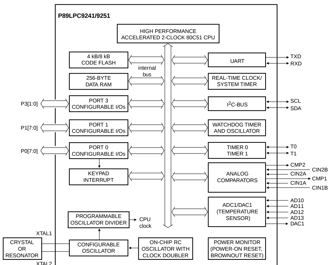
Fig 2. Block diagram (P89LPC9241/9251)
