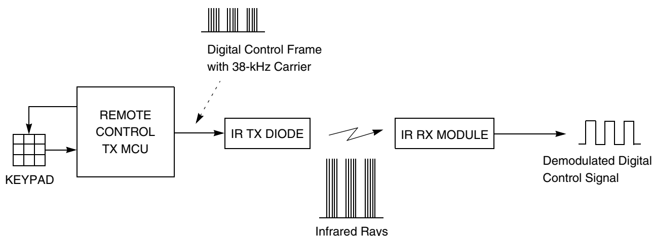
Figure 2-1. Configuration of IR Remote Control Unit
