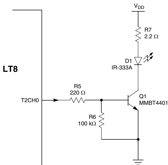
Figure 4-5. Circuit for IR Transmitting Diode
