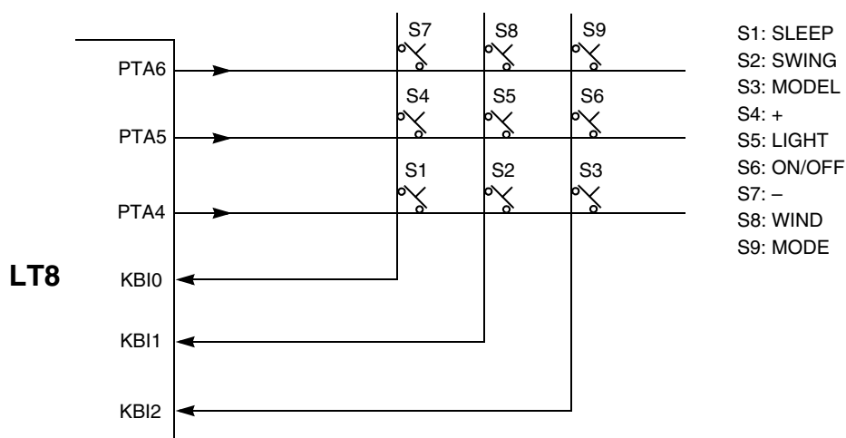
Figure 4-2. Transmitter 3-by-3 Keyboard Matrix
