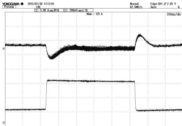
Figure 7: Dynamic response to load step 25%~75% with 0.1A/uS slew rate at 110/220Vac TOP: Vout, 200mV/div, BOTTOM: Iout, 5A/div, 200uS/div
