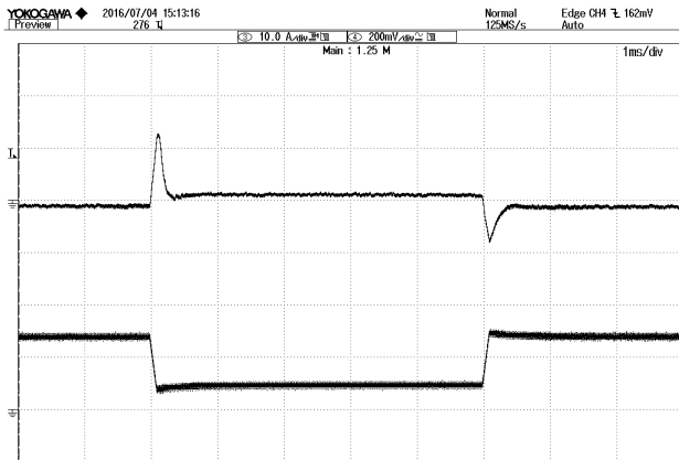
Figure 4: Dynamic response to load step 3A~9A with 0.1A/uS slew rate at 110/220Vac TOP: Vout, 200mV/div, BOTTOM: Iout, 10A/div, 1ms/div
