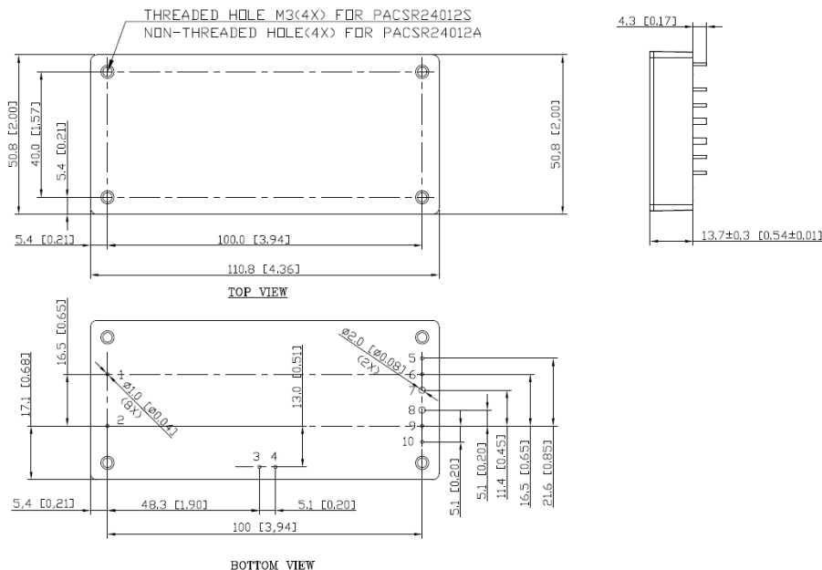
Mechanical Dimensions
