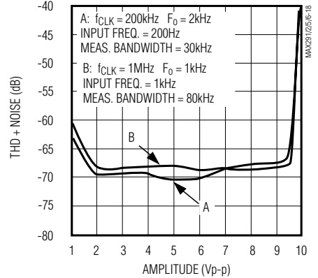
MAX296 THD + NOISE vs. INPUT SIGNAL AMPLITUDE
