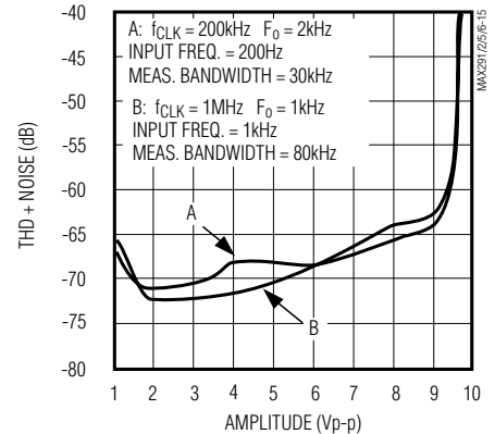
MAX291 THD + NOISE vs. INPUT SIGNAL AMPLITUDE
