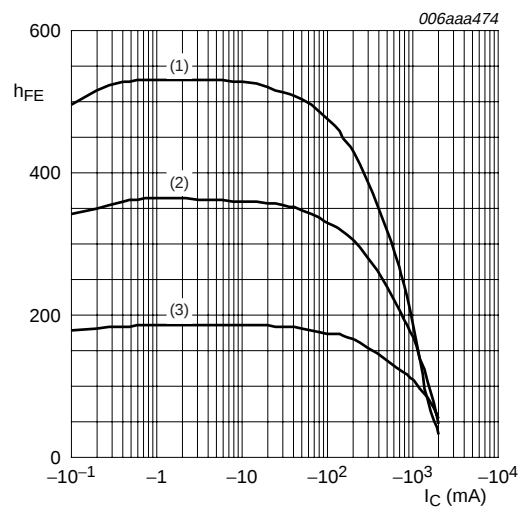
V_{CE} = -5\text{ V} (1) T_{amb} = 100^\circ\text{C} (2) T_{amb} = 25^\circ\text{C} (3) T_{amb} = -55^\circ\text{C}
