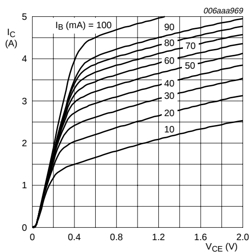
T_{amb} = 25 °C
