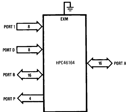
FIGURE 15. Single-Chip Mode
