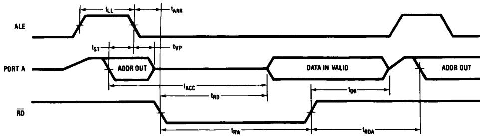
FIGURE 5. Read Cycle
