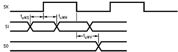
FIGURE 8. MICROWIRE Setup/Hold Timing
