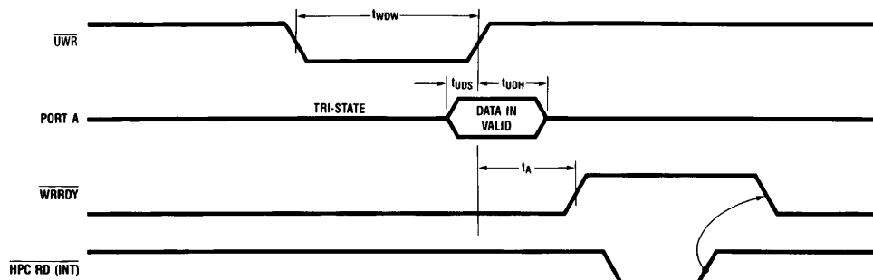
FIGURE 10. UPI Write Timing
