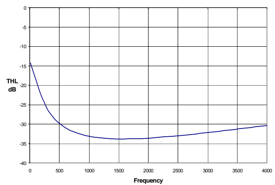
Figure 12. Trans-Hybrid Loss
