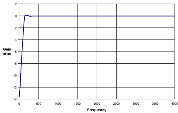
Figure 8. Receive Frequency Response at RX
