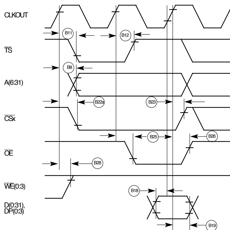
Figure 7. External Bus Read Timing Diagram (GPCM Controlled—ACS = '00')
