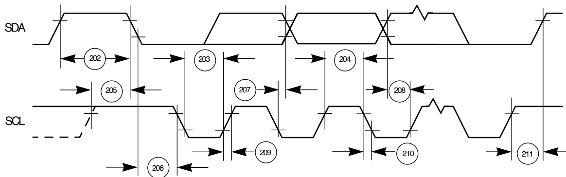
Figure 56. I²C Bus Timing Diagram
