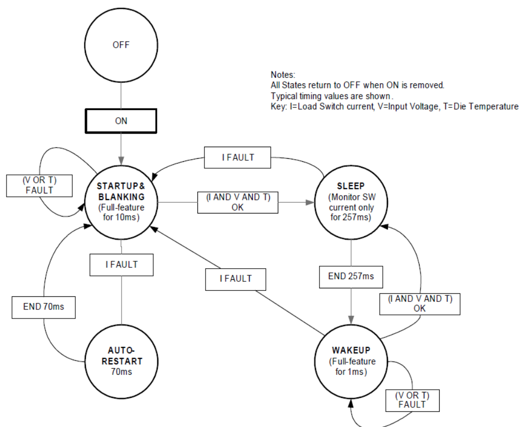
Figure 25. State Diagram with Blanking and Auto-Restart (PPF2024/5)
