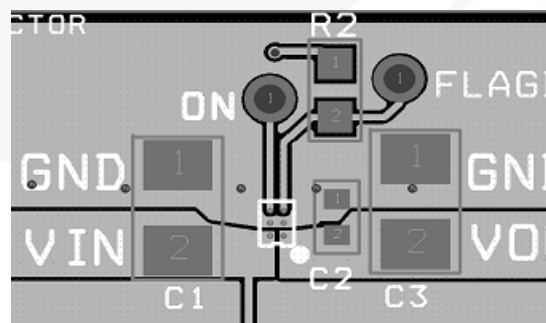
Figure 28. PPF2020X Proper Layout
