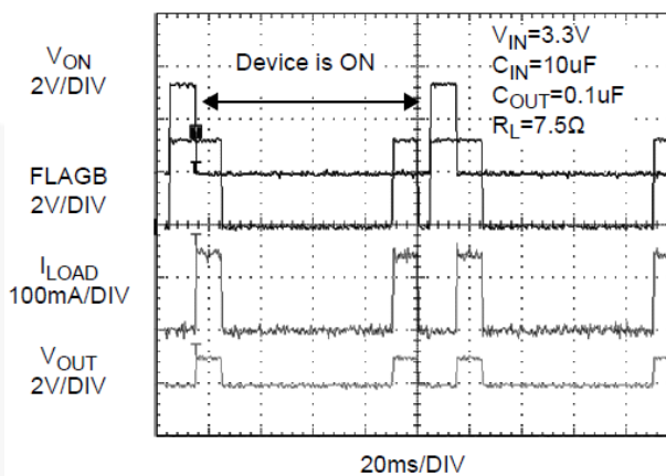
Figure 24. PPF2025 T_{BLANK} and T_{RESTART} (Active LO Device)
