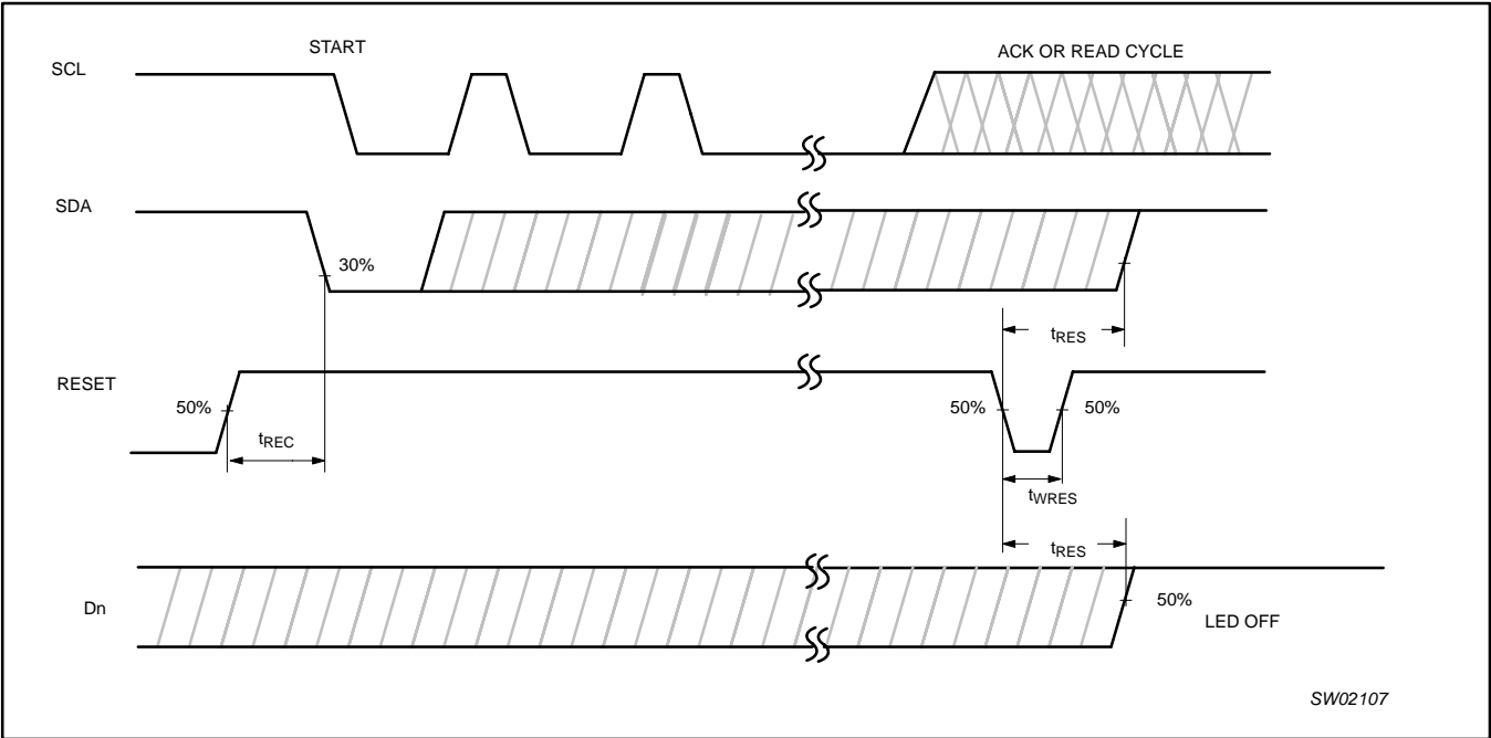
Figure 19. Reset timing
