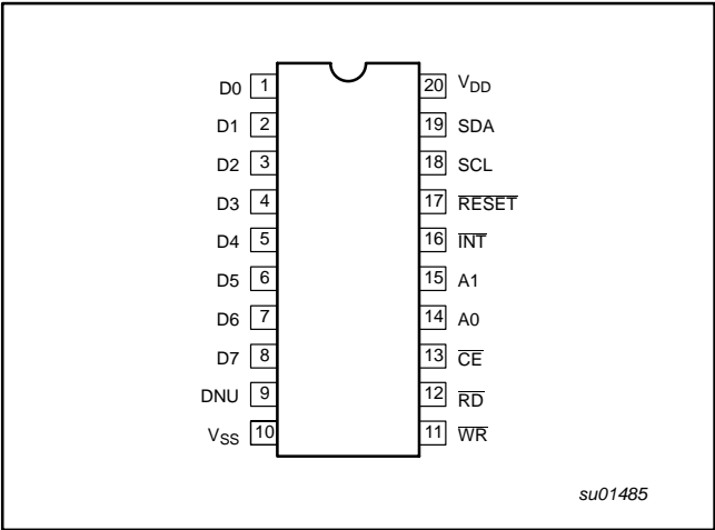
PIN CONFIGURATION
