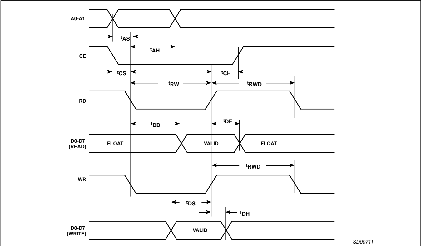
Figure 20. Bus timing
