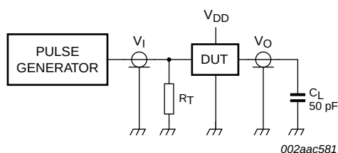
Fig 16. Test circuitry for switching times, SDOUT ( t_v(\text{SDOUT}) )
