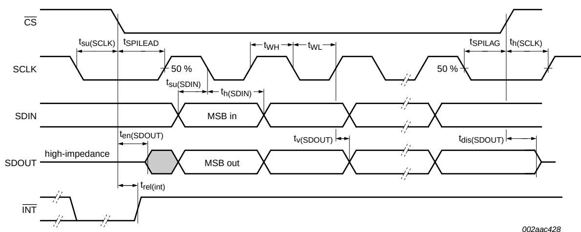
Fig 12. Timing diagram
