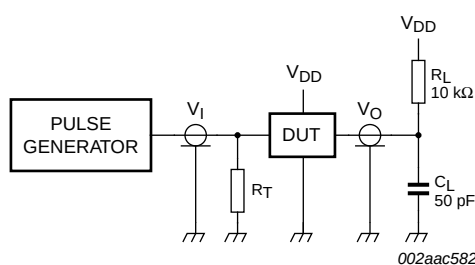
Fig 17. Test circuitry for switching times, \overline{\text{INT}}
