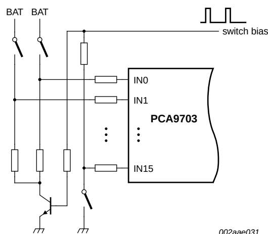
Fig 11. Switches to battery and ground with cyclic biasing
