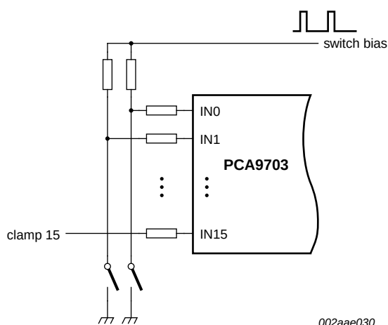
Fig 10. Clamp 15 (ignition) detection
