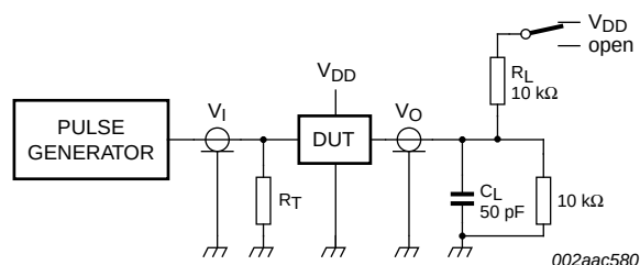
Fig 15. Test circuitry for enable/disable times, SDOUT ( t_{\text{en}}(\text{SDOUT}) and t_{\text{dis}}(\text{SDOUT}) )
