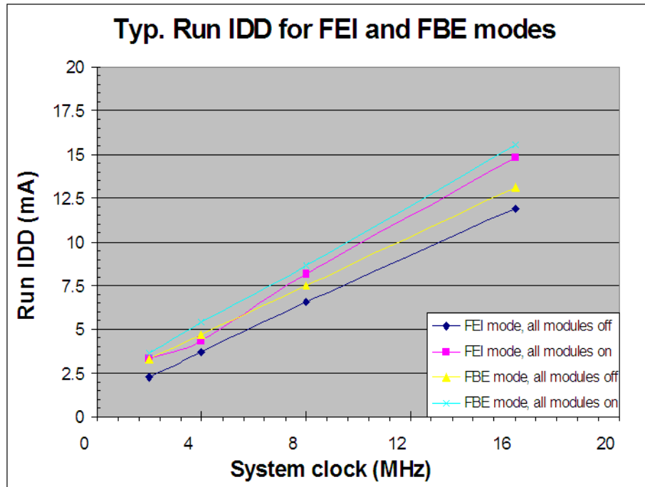
Figure 8. Typical Run I_{DD} vs. System Clock Freq. for FEI and FBE Modes
