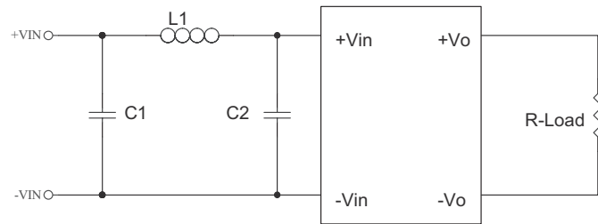
Figure 3 Conducted Emissions Test Circuit
