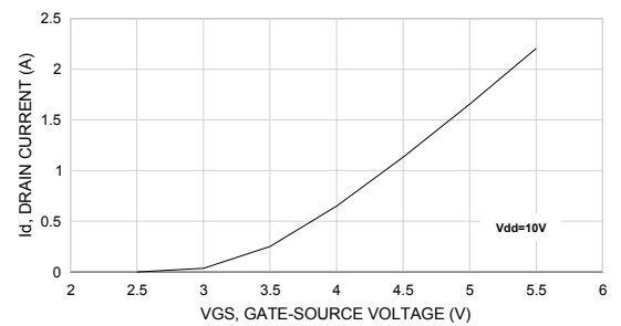
Figure 4. Drain current vs gate-source voltage
