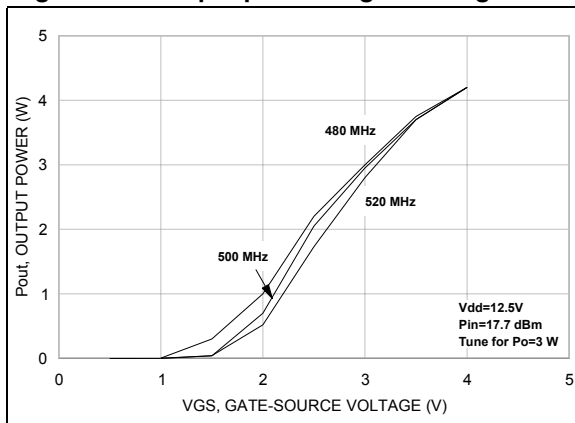
Figure 26. Output power vs gate voltage
