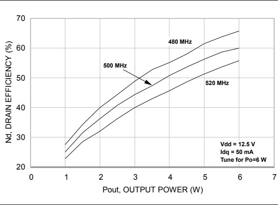
Figure 9. Drain efficiency vs output power
