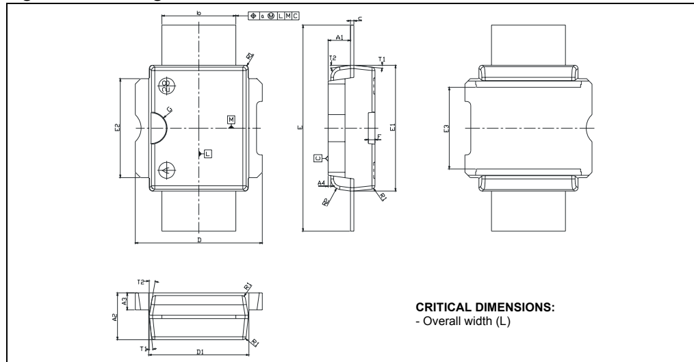
Figure 34. Package dimensions
