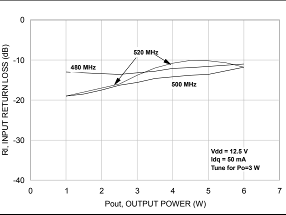
Figure 11. Return loss vs output power
