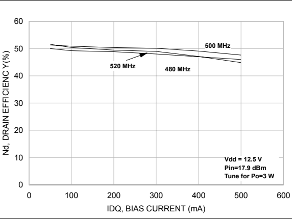
Figure 13. Drain efficiency vs bias current
