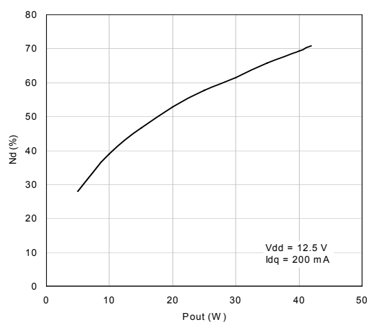
Figure 18. Drain efficiency vs output power (f = 175 MHz)
