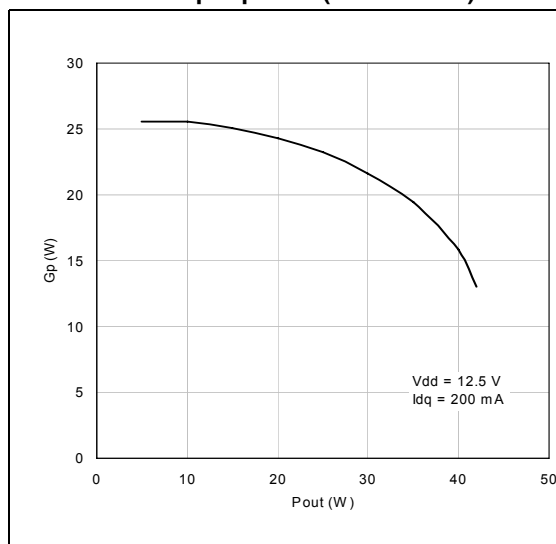
Figure 17. Power gain vs output power (f = 175 MHz)
