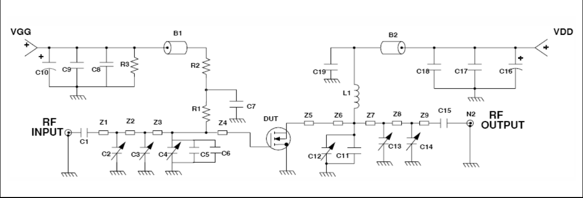
Figure 20. 500 MHz test circuit schematic (engineering)
