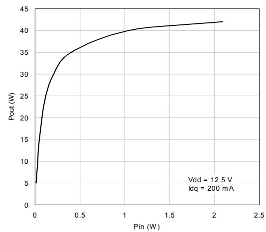
Figure 16. Output power vs input power (f = 175 MHz)
