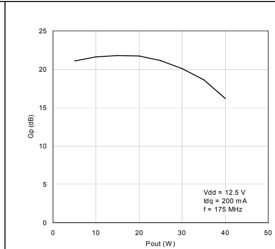
Figure 17. Power gain vs output power
