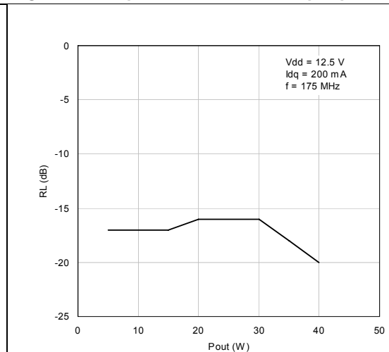
Figure 19. Input return loss vs output power
