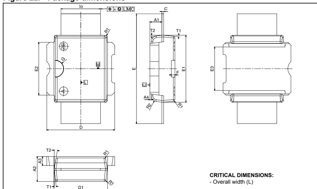
Figure 22. Package dimensions
