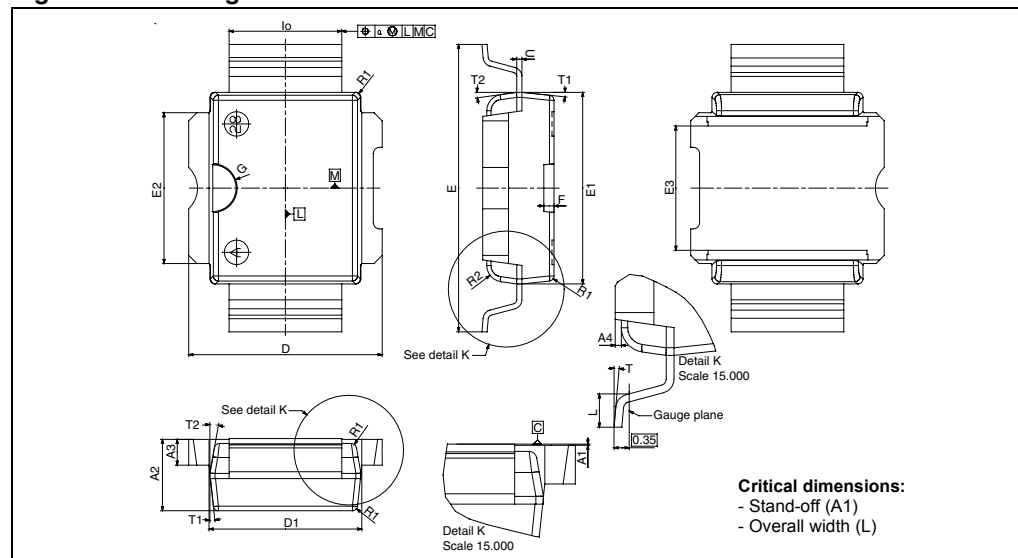
Figure 21. Package dimensions
