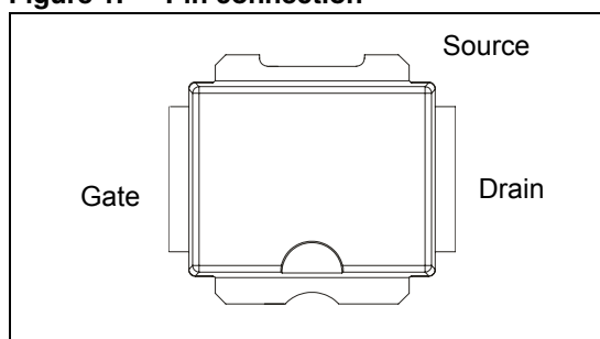
Figure 1. Pin connection
