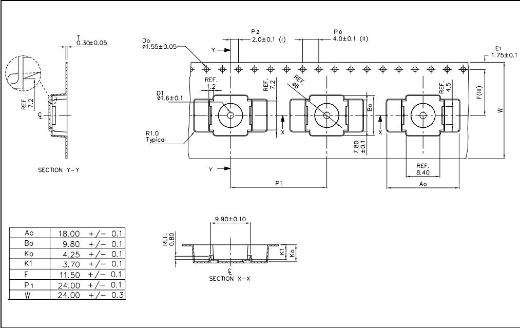
Figure 24. Reel information
