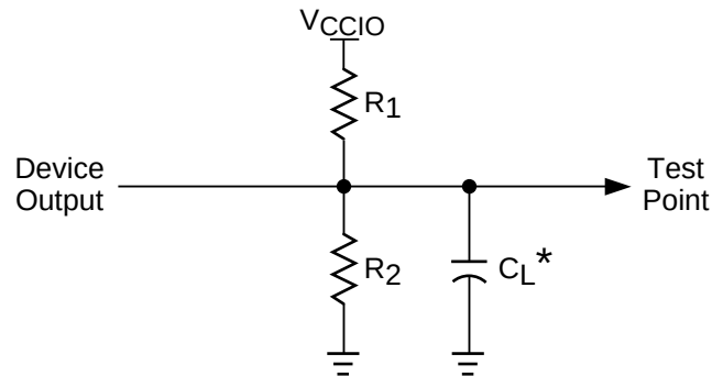
Figure 9. Test Load
