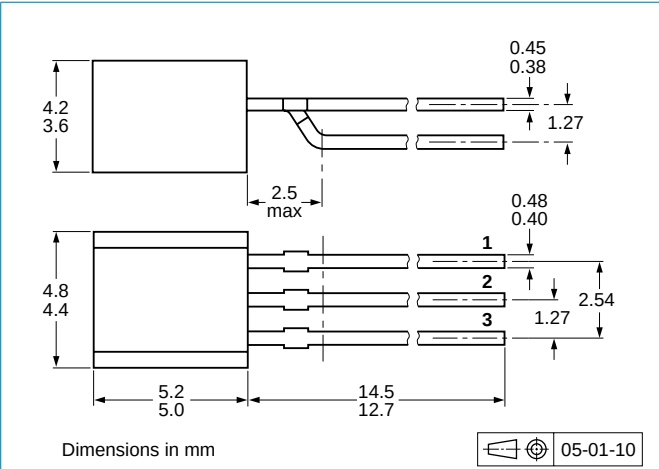
Fig 11. Package outline SOT54 variant
