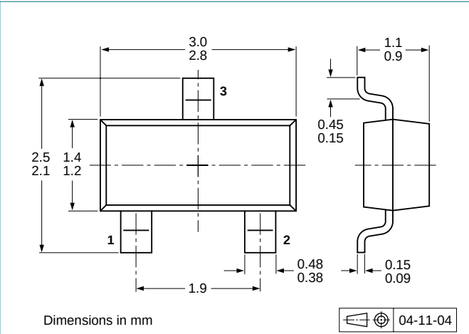
Fig 12. Package outline SOT23 (TO-236AB)
