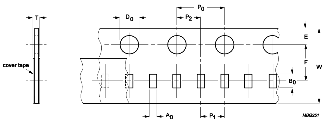
Fig. 7 Paper Tape
