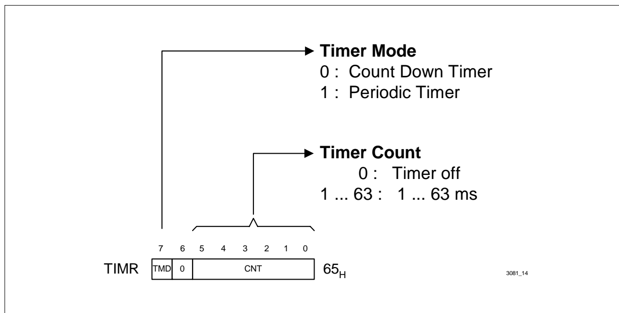
Figure 11 Timer Register
