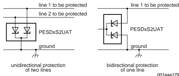
Fig.10 Typical application: ESD protection of data lines.
