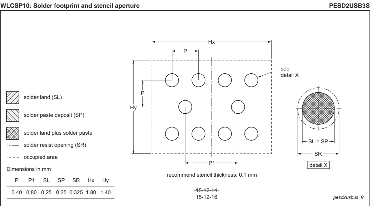
Fig 19. Soldering footprint WLCSP10 (PESD2USB3S)
