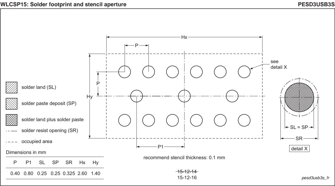
Fig 20. Soldering footprint WLCSP15 (PESD3USB3S)
