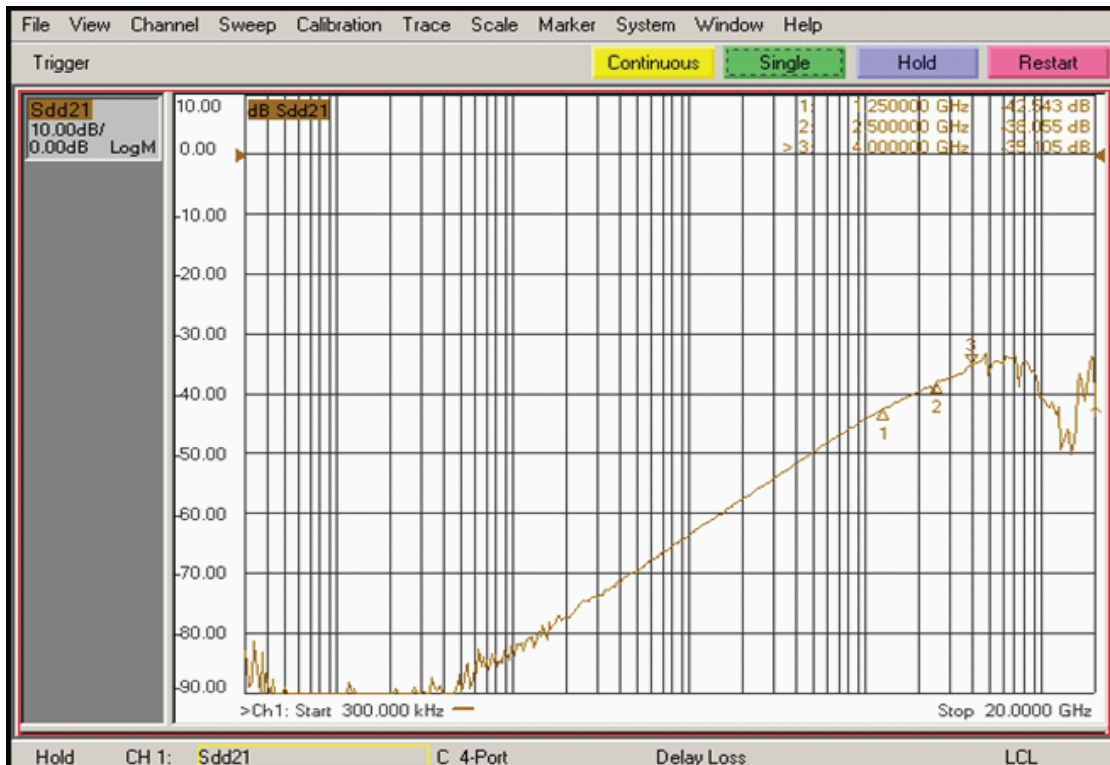
Differential Crosstalk
