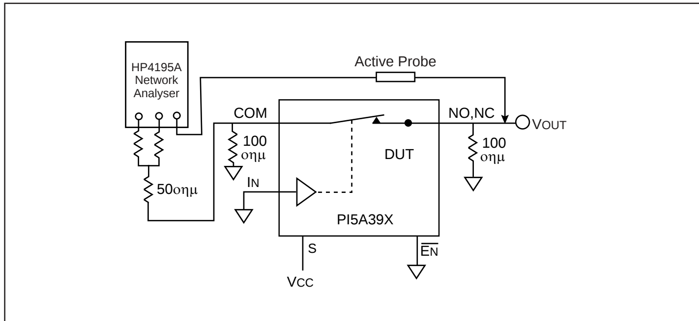
Figure 3. Bandwidth
