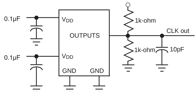
Test Circuit 2
