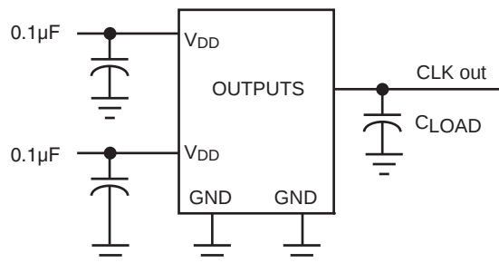
Test Circuit 1
