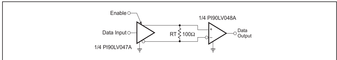
Figure 5. Point-to-Point Application
