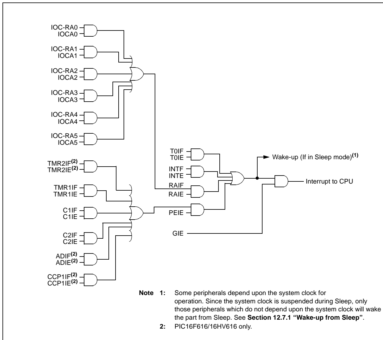
FIGURE 12-7: INTERRUPT LOGIC
