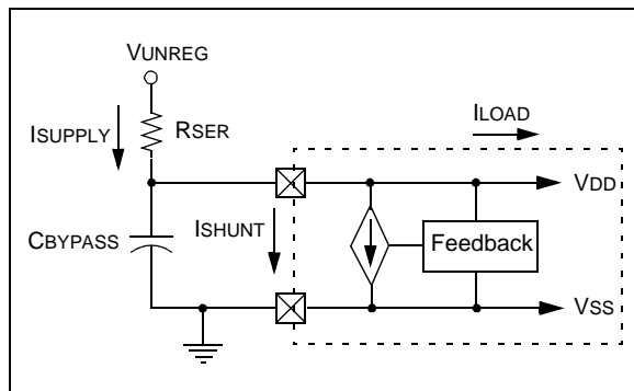
FIGURE 11-1: VOLTAGE REGULATOR
