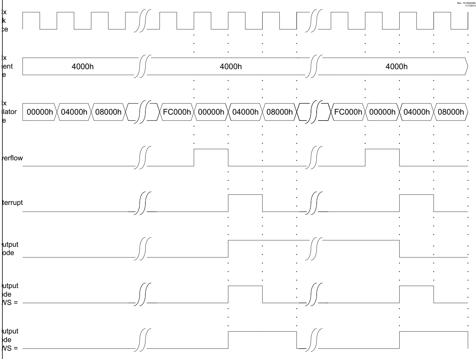
FIGURE 24-2: FDC OUTPUT MODE OPERATION DIAGRAM
