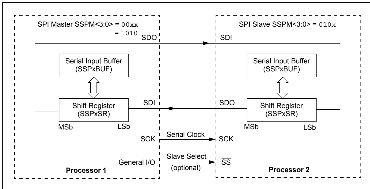
FIGURE 31-5: SPI MASTER/S�AVE CONNECTION
