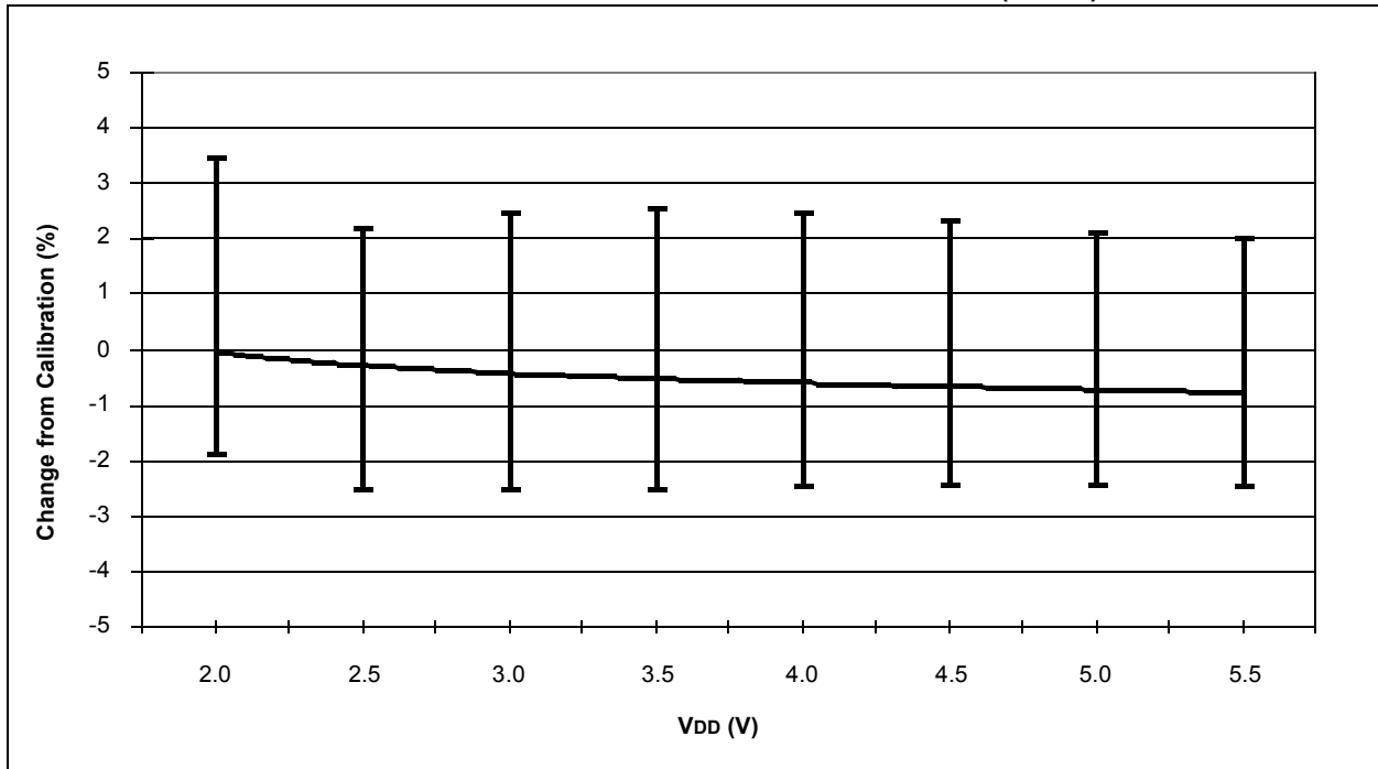
FIGURE 18-41: TYPICAL HFINTOSC FREQUENCY CHANGE vs. V_{DD} ( 125^{\circ}\text{C} )
