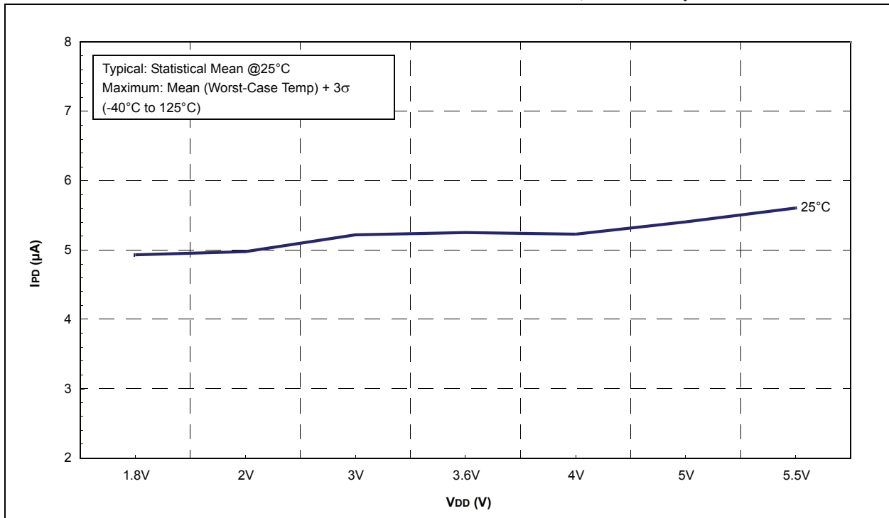
FIGURE 24-29: PIC16F722A/723A TYPICAL BASE I_{PD} vs. V_{DD} , V_{CAP} = 0.1\mu F
