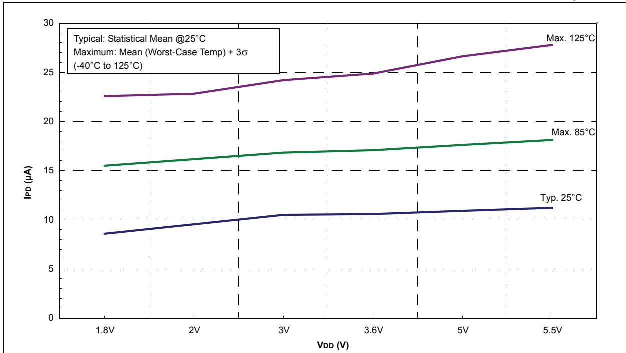
FIGURE 24-37: PIC16F722A/723A CAP SENSE MEDIUM POWER I_{PD} vs. V_{DD} , V_{CAP} = 0.1\mu F
