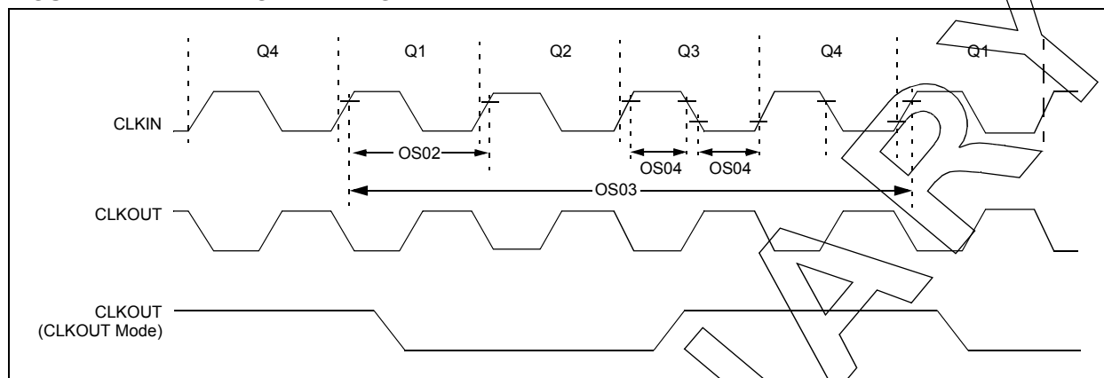
FIGURE 22-4: CLOCK TIMING
