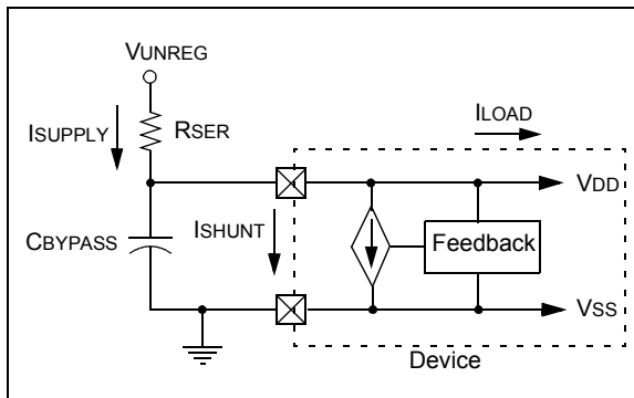
FIGURE 20-1: SHUNT REGULATOR
