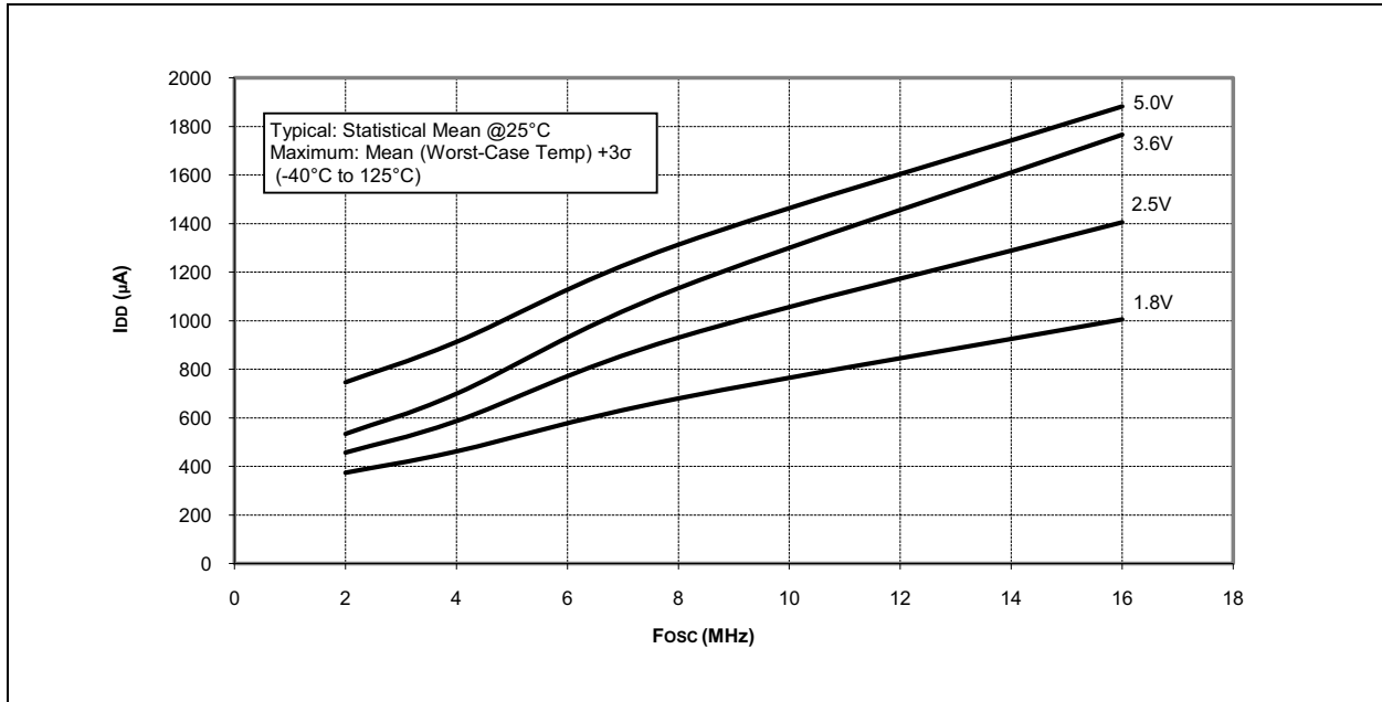
FIGURE 24-9: PIC16F720/721 MAX. I DD vs. F osc OVER V DD , HFINTOSC
