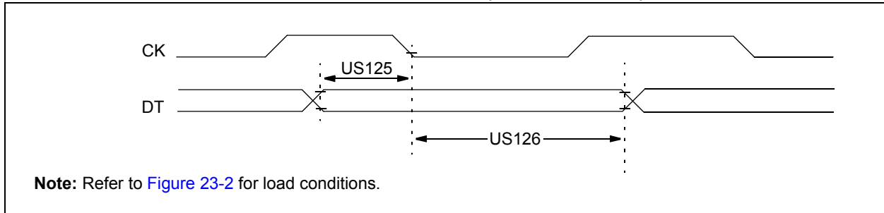
FIGURE 23-14: USART SYNCHRONOUS RECEIVE (MASTER/S�AVE) TIMING
