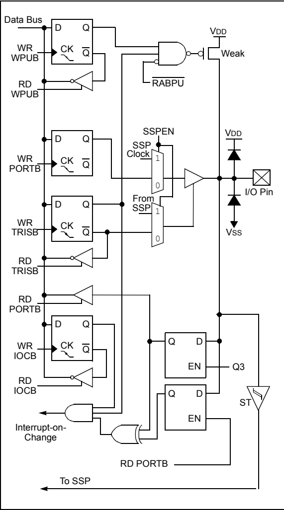
FIGURE 6-9: BLOCK DIAGRAM OF RB6
