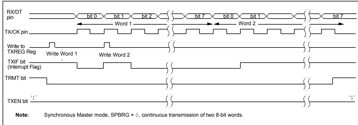
FIGURE 16-6: SYNCHRONOUS TRANSMISSION
