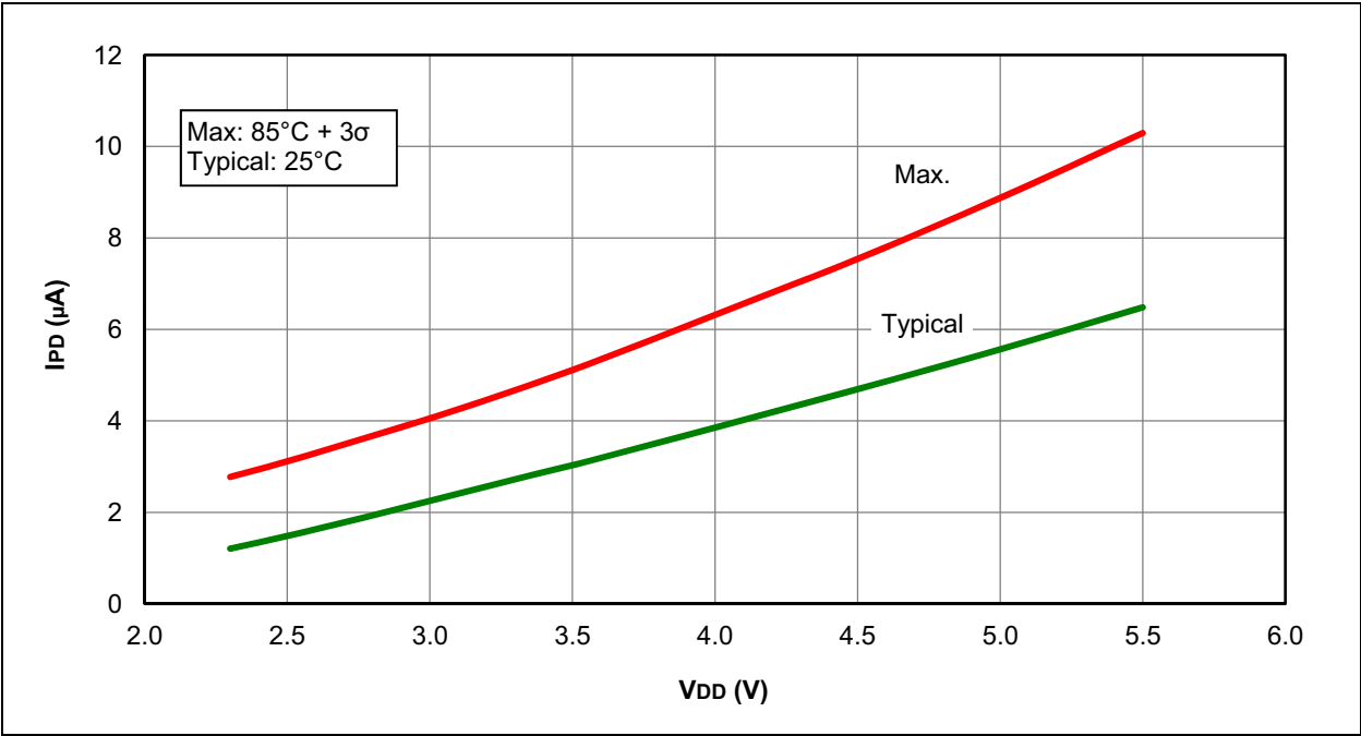
FIGURE 26-40: I_{PD} , SECONDARY OSCILLATOR, F_{osc} = 32\text{ kHz} , PIC16F1526/7 ONLY
