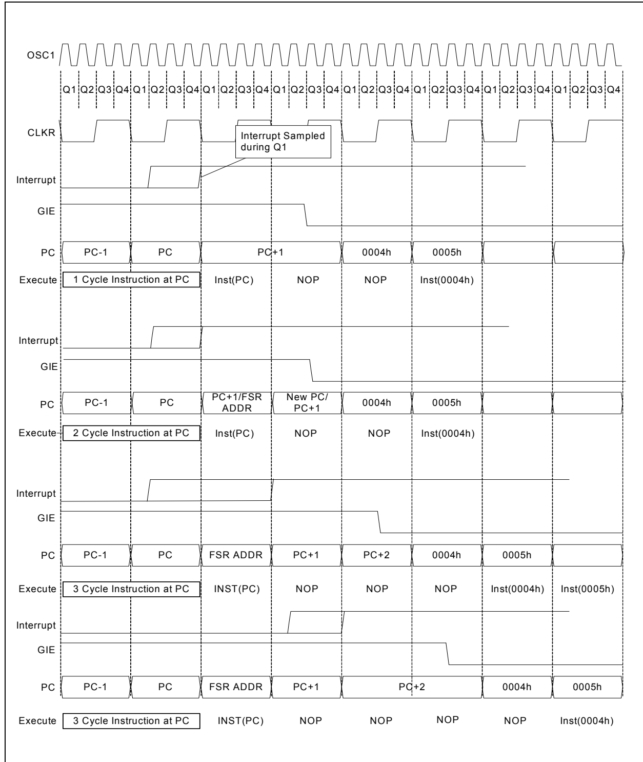
FIGURE 7-2: INTERRUPT LATENCY
