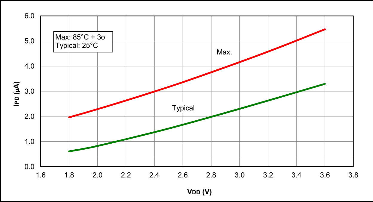
FIGURE 26-39: I_{PD} , SECONDARY OSCILLATOR, F_{osc} = 32\text{ kHz} , PIC16LF1526 ONLY
