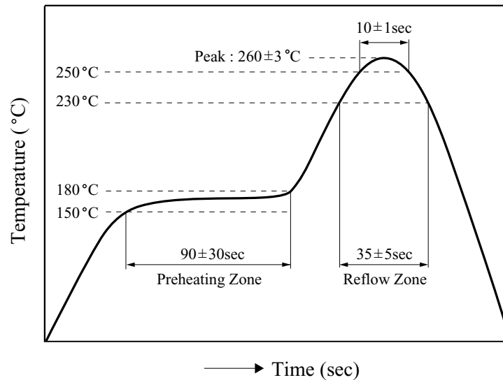
[Lead-Free Soldering Temperature Profile]
