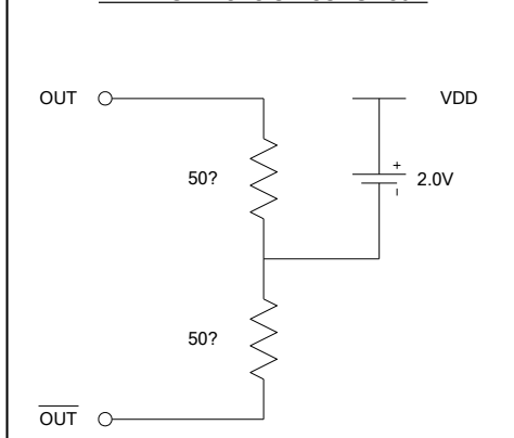
LVPECL Levels Test Circuit
