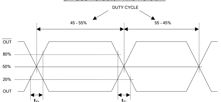
LVPECL Transistion Time Waveform
